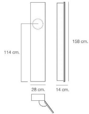
Armario 156 cm. - espejo frontal (dch.) / Decapé Wall cabinet 156 cm. with front mirror (right) / Light Oak 51.54.07.250
