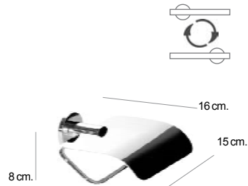
Portarrollos c/tapa Paper holder ○ 41.40.03.002
