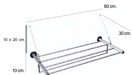
Estanteria toallas Towel rack ○ 41.51.10.002
