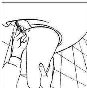
6 Position trap cover under the lavatory, pull down the spring and attach each spring into the hole on each side of the trap cover.
