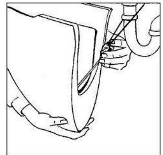
8 Pass the screw tap through the hole beneath the trap cover.
