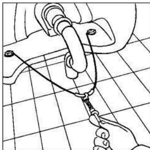
5 Center the screw.
