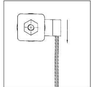
4 When the fixing process is over, the direction of the nut should be downwards, not left or right.
